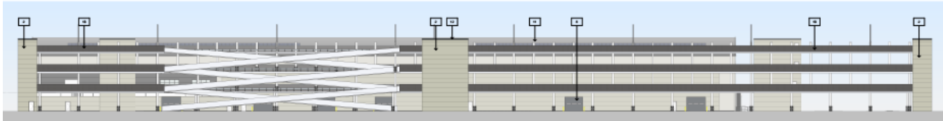
E03 - SOUTH ELEVATION
